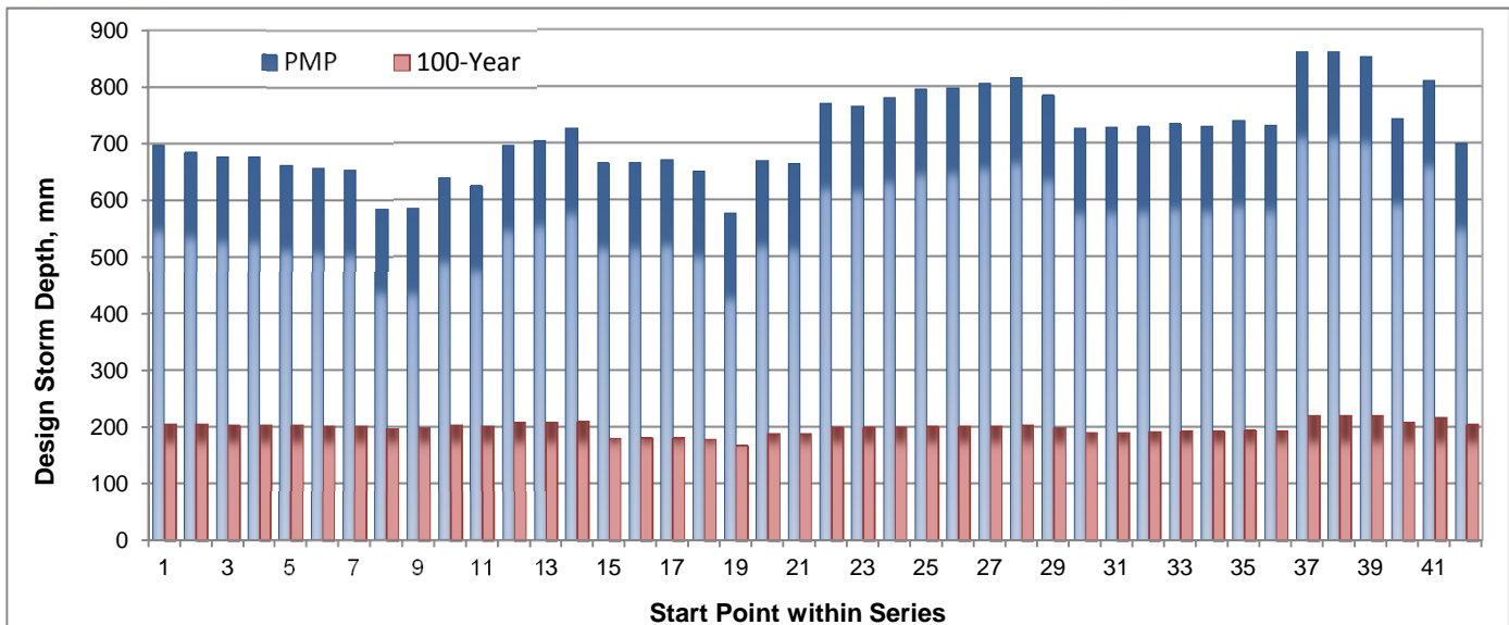
Figure B.4(b): Variation in PMP and 100-Year Estimates for Central America Record Resampled in 20-Year Segments
