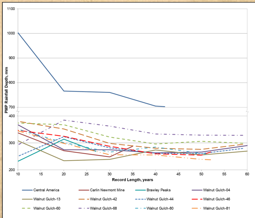
PMP vs. Record Length
