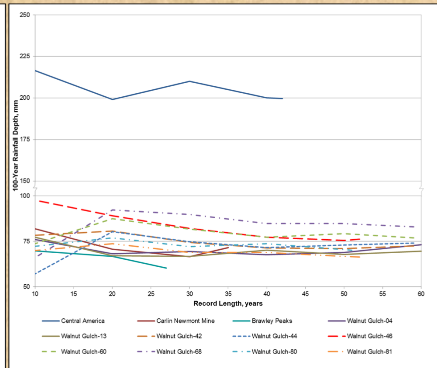
100-yr Storm vs. Record Length
